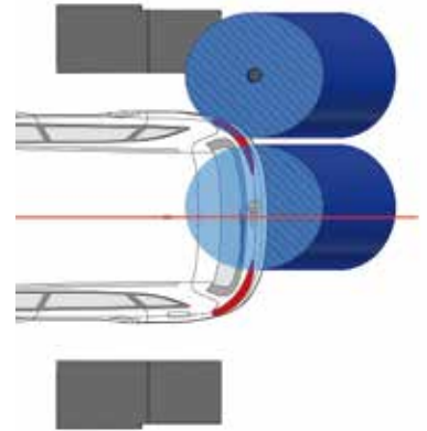
Comprehensive centre cross-over wash with inclined brushes
